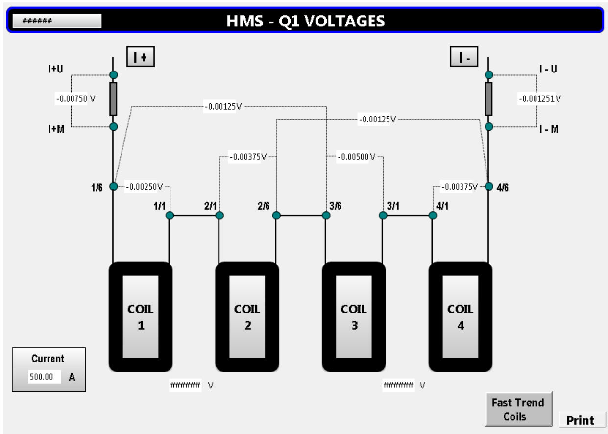
HMS Quadrupole 1 Voltages CSS-BOY screen
